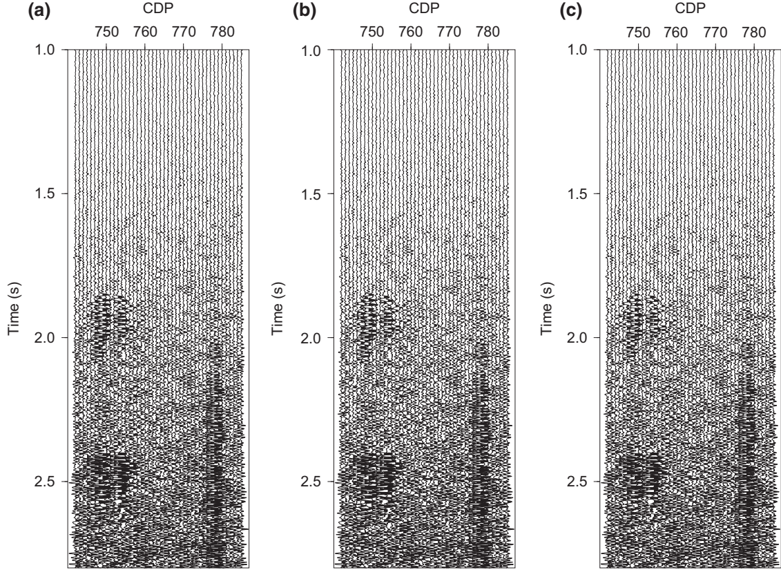
Figure 11 The comparison of the difference sections of three different methods in the right rectangular window highlighted in Fig. 5a. Difference sections of (a) robust f - x projection, (b) f - x deconvolution, and (c) least-squares f - x projection.
