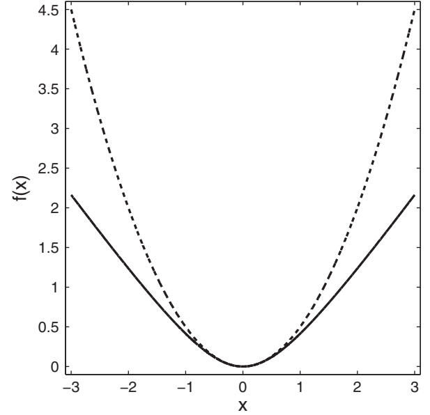
Figure 2 The dashed line represents the quadratic function \frac{1}{2}|x|^2 . The solid line represents the hybrid function \sqrt{1+|x|^2} - 1 .
