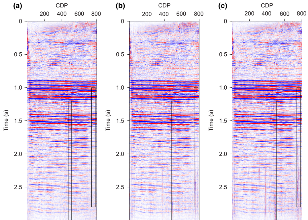
Figure 6 (a) Data after robust f - x projection filtering. (b) Data after f - x deconvolution filtering. (c) Data after least-squares f - x projection filtering.
