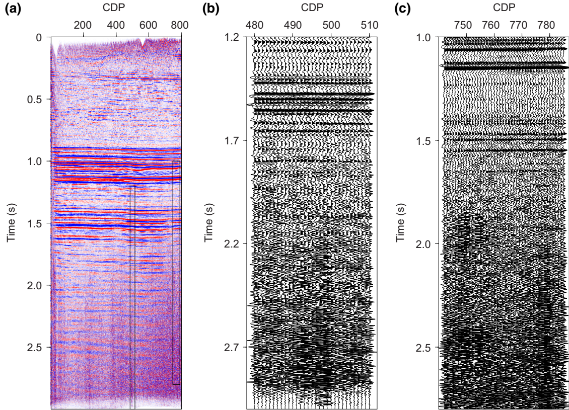
Figure 5 (a) Poststack data from WCSB with erratic noise and random Gaussian noise. (b) The data in the left rectangular window. (c) The data in the right rectangular window.
