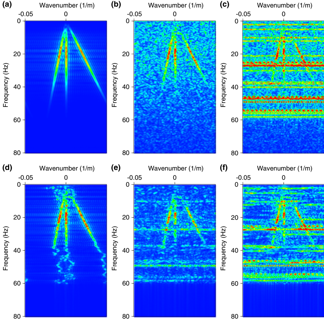
Figure 4 (a) f - k spectrum of noise-free data. (b) f - k spectrum of data corrupted with Gaussian noise. (c) f - k spectrum of the input noisy data (Fig. 3a). (d) f - k spectrum of robust f - x projection filtered data (Fig. 3d). (e) f - k spectrum of f - x deconvolution filtered data (Fig. 3e). (f) f - k spectrum of least-squares f - x projection filtered data (Fig. 3f).
