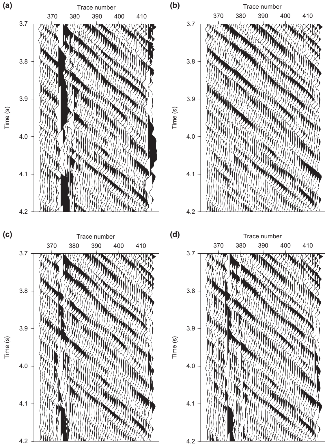
Figure 16 (a) The data in the right rectangular window highlighted in Fig. 12a. (b) The result of robust f - x projection. (c) The result of f - x deconvolution. (d) The result of least-squares f - x projection.
