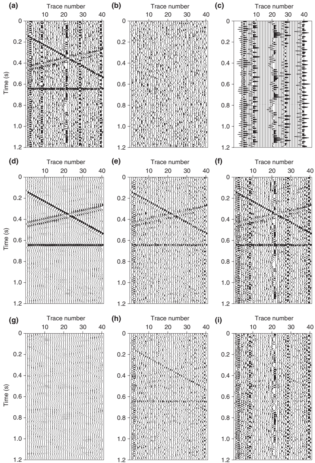
Figure 3 (a) Noisy synthetic data (after clipping). (b) Gaussian noise with \text{SNR} = 1.2 . (c) Erratic noise. (d) Denoising via robust f - x projection. (e) Denoising via f - x deconvolution. (f) Denoising via least-squares f - x projection. (g) Difference section for robust f - x projection. (h) Difference section for f - x deconvolution. (i) Difference section for least-squares f - x projection filter.
