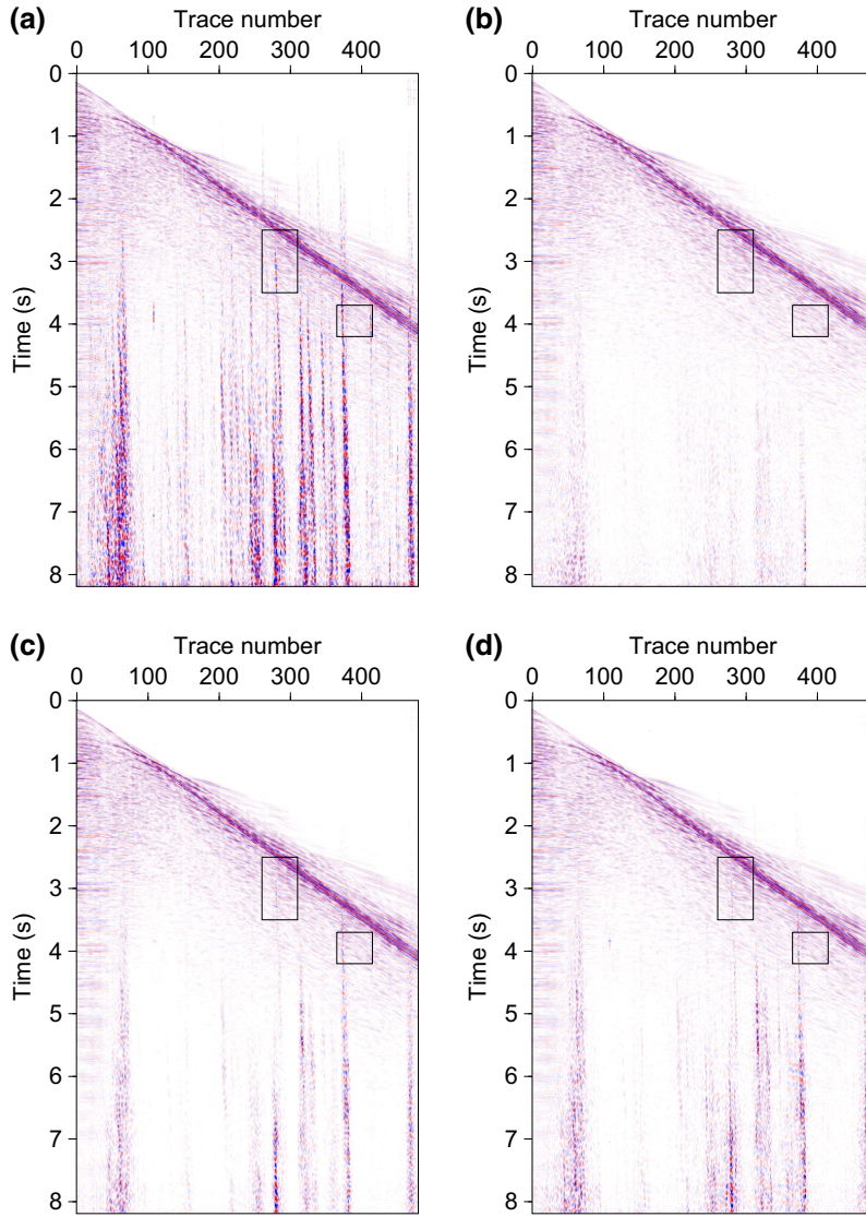
Figure 12 (a) Input marine shot gather with strong swell noise. (b) Data after robust f - x projection filtering. (c) Data after f - x deconvolution filtering. (d) Data after least-squares f - x projection filtering.
