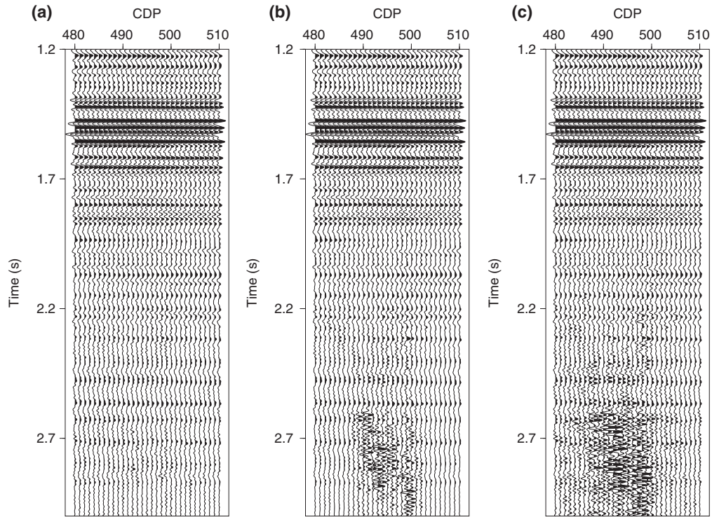
Figure 8 The comparison of the filtered results of the data in the left rectangular window highlighted in Fig. 5a. (a) The result of robust f-x projection. (b) The result of f-x deconvolution. (c) The result of least-squares f-x projection.
