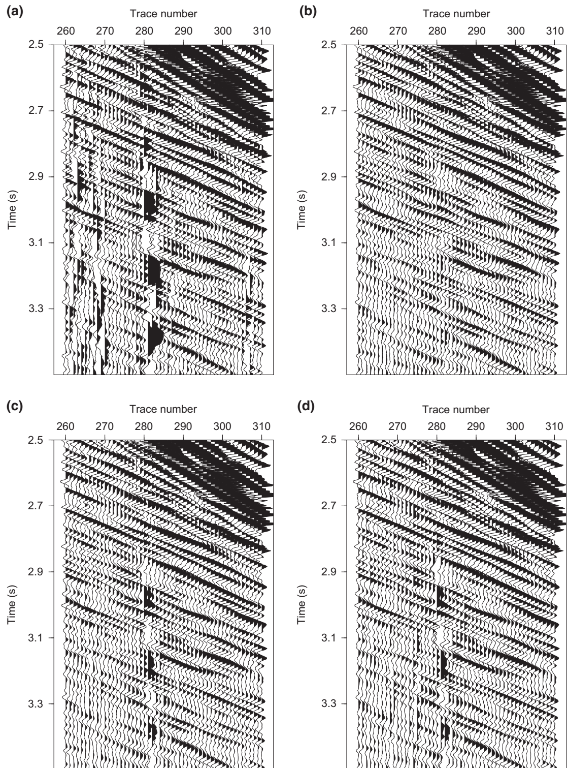
Figure 14 (a) The data in the left rectangular window highlighted in Fig. 12a. (b) The result of robust f - x projection. (c) The result of f - x deconvolution. (d) The result of least-squares f - x projection.
