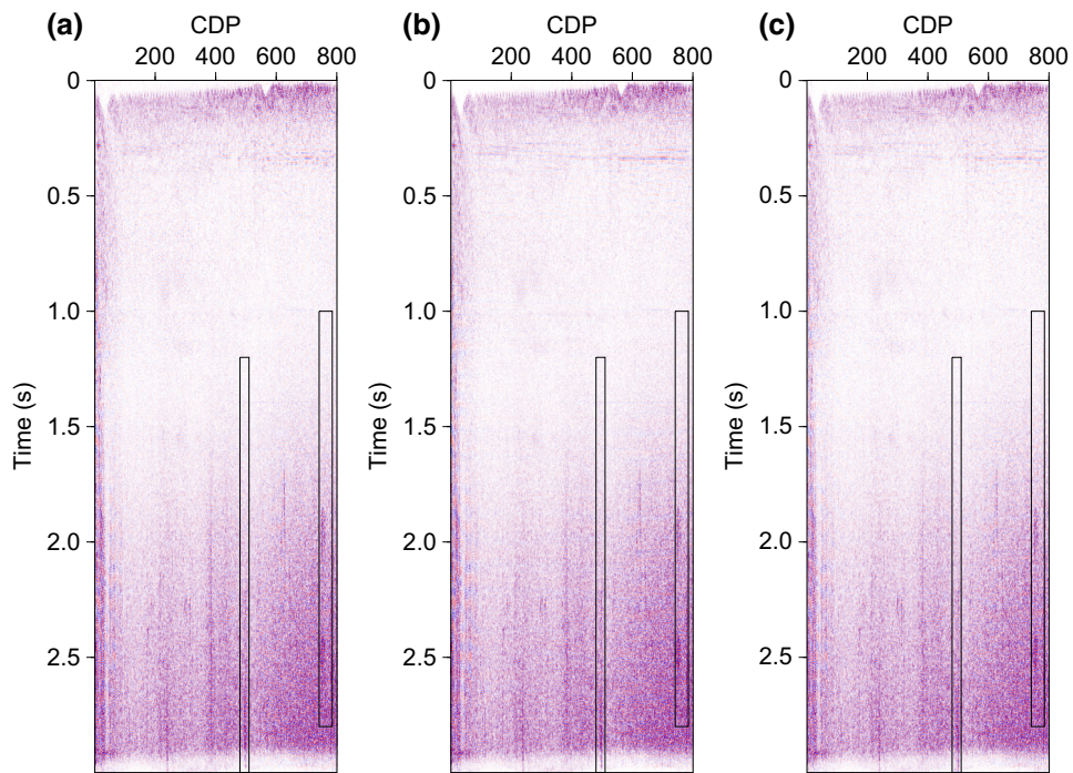
Figure 7 Difference sections (input noisy data minus filtered data) of (a) robust f - x projection, (b) f - x deconvolution, and (c) least-squares f - x projection.
