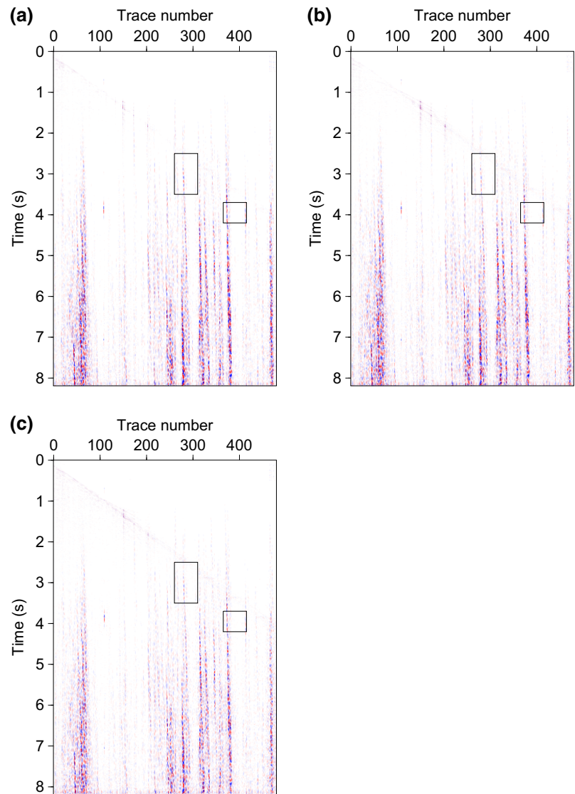
Figure 13 Difference sections of (a) robust f - x projection, (b) f - x deconvolution, and (c) least-squares f - x projection.
