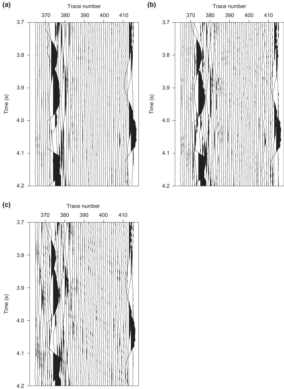
Figure 17 The comparison of the difference sections of three different methods in the right rectangular window highlighted in Fig. 12a. Difference sections of (a) robust f - x projection, (b) f - x deconvolution, and (c) least-squares f - x projection.
