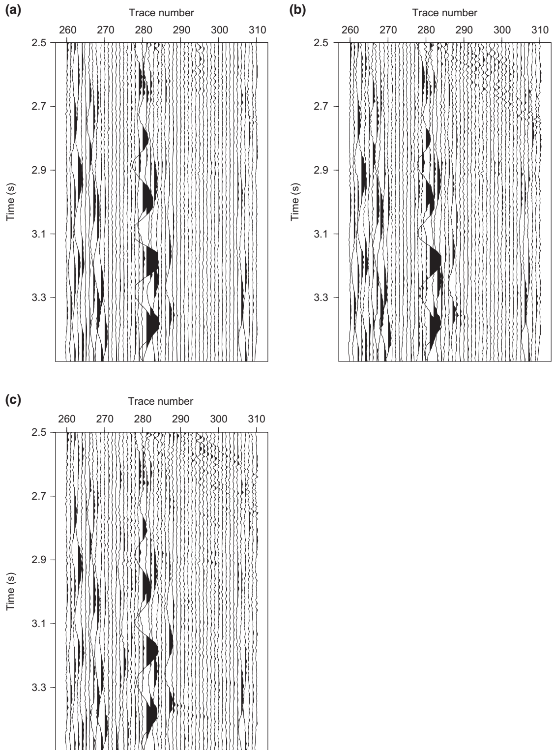
Figure 15 The comparison of the difference sections of three different methods in the left rectangular window highlighted in Fig. 12a. Difference sections of (a) robust f - x projection, (b) f - x deconvolution, and (c) least-squares f - x projection.
